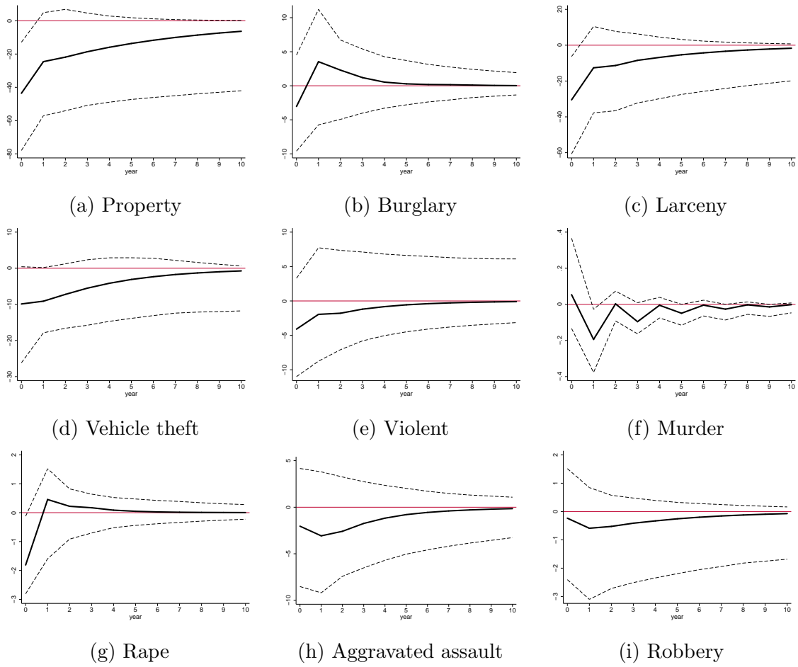
Figure 6: Evolution of effect of one-off $100 dividend increase (number of crimes per 100,000 population, with 95% prediction intervals), with conditionality. Estimated using ARDL(2,1) model.
