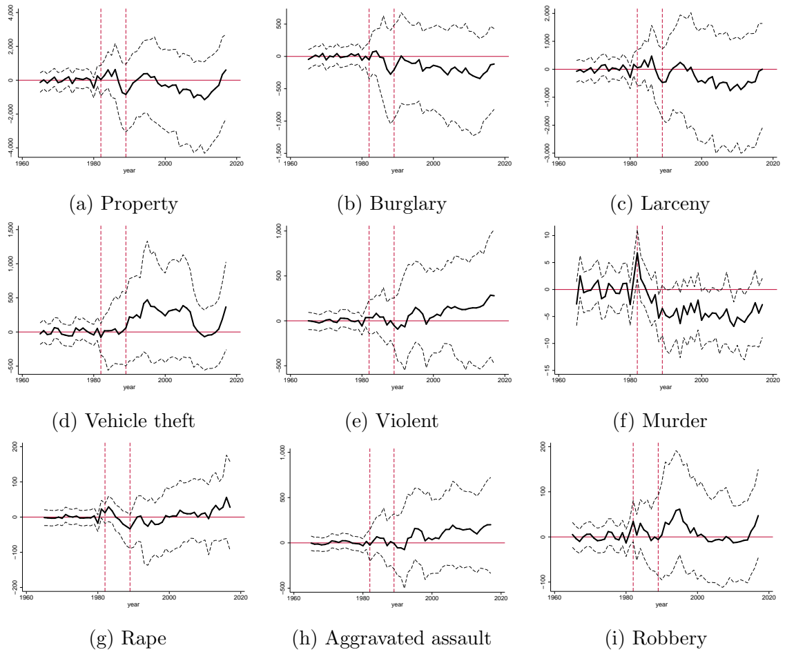
Figure 4: Impacts of the dividend on crime in Alaska using BSTS to construct counterfactual outcomes on the basis of crime trends in other states. In each case, the solid black line shows the impact on the number of crimes per 100,000 population, while the dashed lines are the 95% prediction intervals. Using priors given in Table 2.
