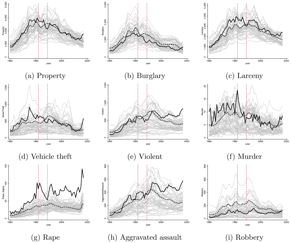
Figure 2: Crime trends in Alaska (solid black line), USA (dash black line) and all other states (grey lines)
