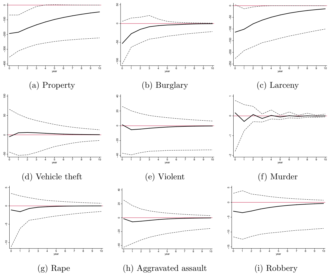
Figure 5: Evolution of effect of one-off $100 dividend increase (number of crimes per 100,000 population, with 95% prediction intervals), without conditionality. Estimated using ARDL(2,1) model.
