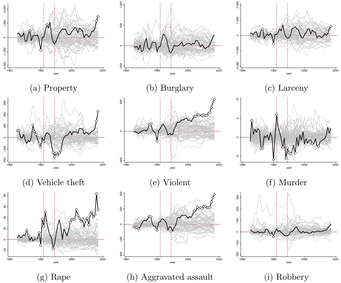
Figure 3: Impacts of eligibility the dividend on crime in Alaska using a synthetic Alaska to represent counterfactual outcomes. In each case, the solid black line shows the difference between Alaska and the synthetic Alaska in the number of crimes per 100,000 population. The thin grey lines are placebo tests for other states. Markers indicate where the Alaskan difference is outside the top or bottom 2.5% of the placebo distribution. Estimates control for the mean pre-1982 rate of the crime in question, rates 1, 3 and 5 years pre-1982 and for state characteristics over those pre-1982 years for which data are available (these characteristics include ratio of convictions to crimes, unemployment rate, educational attainment and income inequality).
