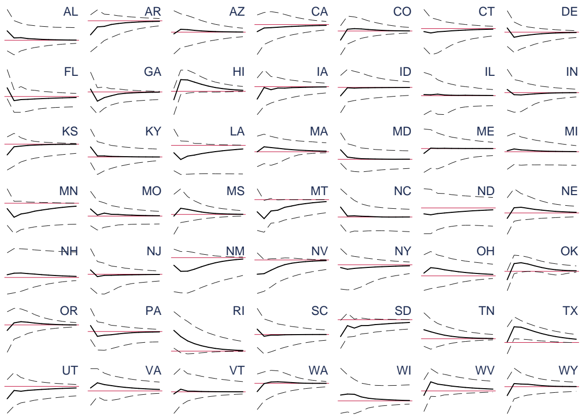
Figure 8: Evolution of effect of one-off Dividend increase on property crime (with 95% credible intervals), with conditionality by state. Estimated using ARDL(2,1) model. For each state, effects for 10 years since impulse are shown.
