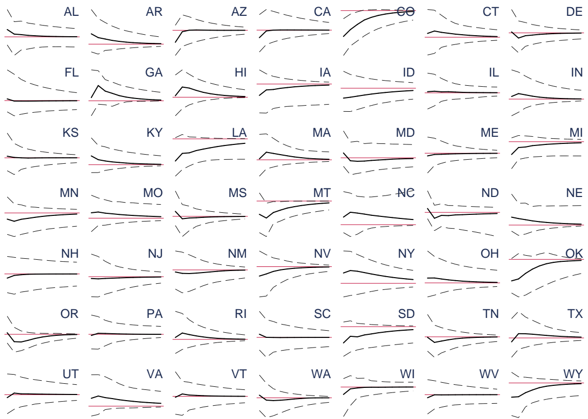
Figure 7: Evolution of effect of one-off placebo Dividend increase on property crime (with 95% credible intervals), without conditionality by state. Estimated using ARDL(2,1) model. For each state, effects for 10 years since impulse are shown.
